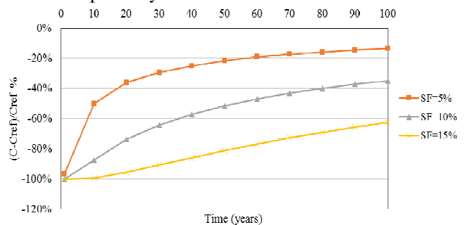
Fig.11: Reduction percentage of chloride concentration at (40, 40) for each value of silica fume with time.
