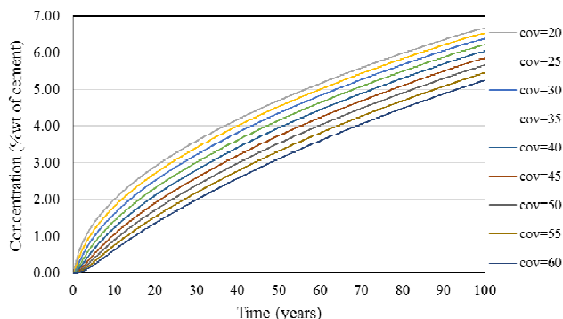
Fig.6: Variation of chloride concentration with time at (cover, cover) for each cover value.
