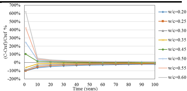
Fig.5: Change percentage of chloride concentration at (40, 40) for different values of w/c ratio with time.
